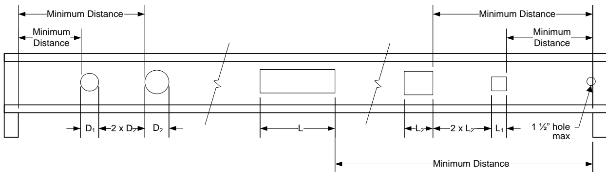
FIGURE 2—HOLE-IN-WEB REQUIREMENTS
